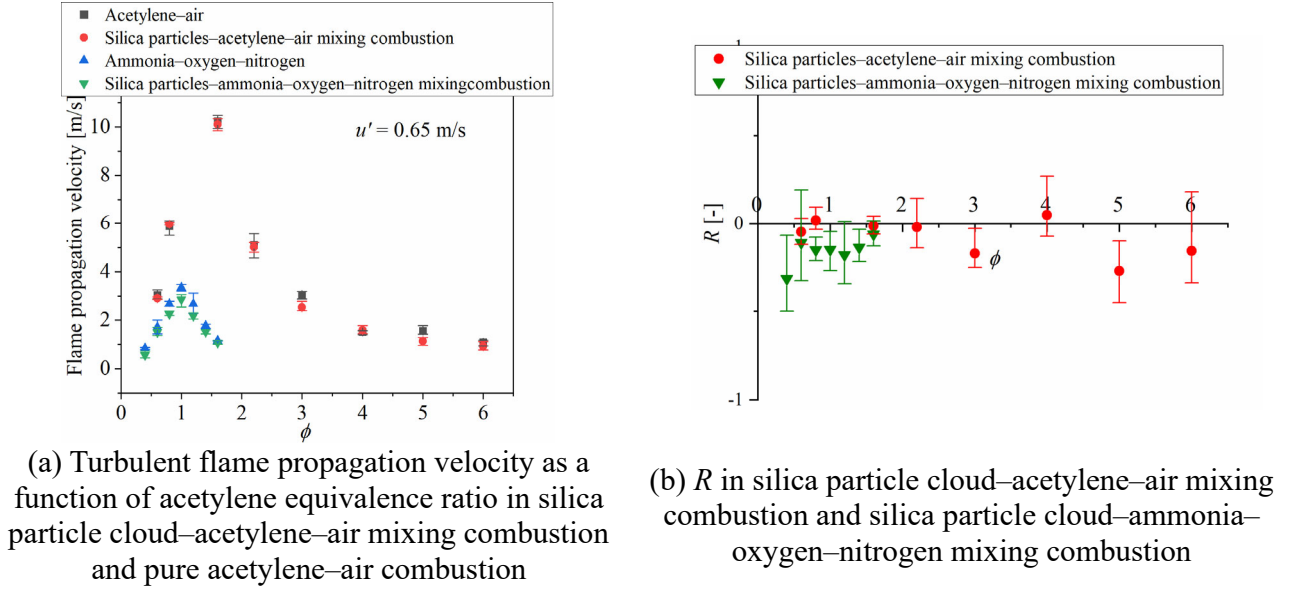
Fig. 8 Turbulent flame propagation in silica particle cloud–acetylene–air mixing combustion and silica particle cloud–ammonia–oxygen–nitrogen mixing combustion.
