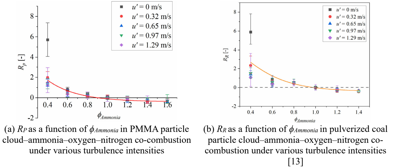
Fig. 10 Impact of particle cloud on pure ammonia combustion with various solid particles.
