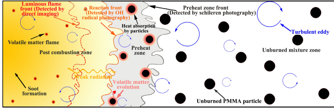
Fig. 11 Turbulent flame structure of PMMA particle cloud–ammonia–oxygen–nitrogen co-combustion.
